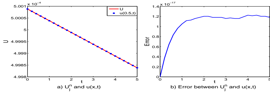
Figure 2: U and u(x,t) at a fixed value x = 0.5 for the NSFD scheme.
