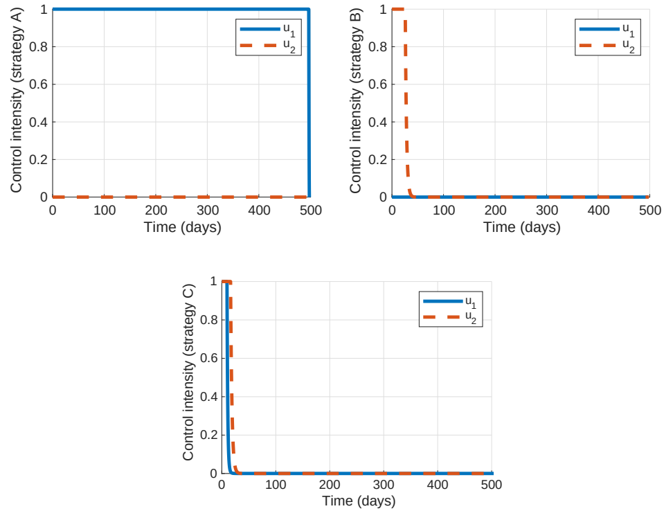
Figure 10: Control profiles for all strategies
