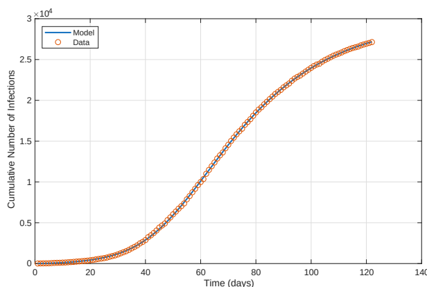
Figure 2: Comparison of model simulation and reported data for cumulative Mpox infections over time
