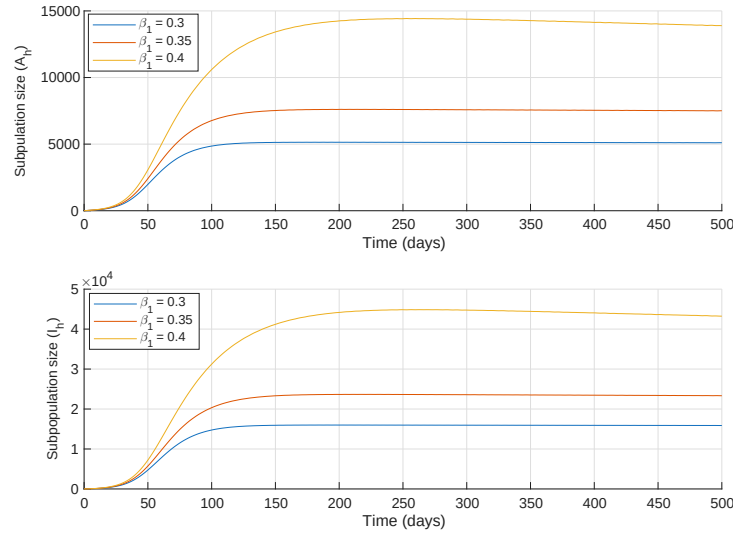
Figure 4: Influence of parameter \beta_1 with respect to A_h and I_h
