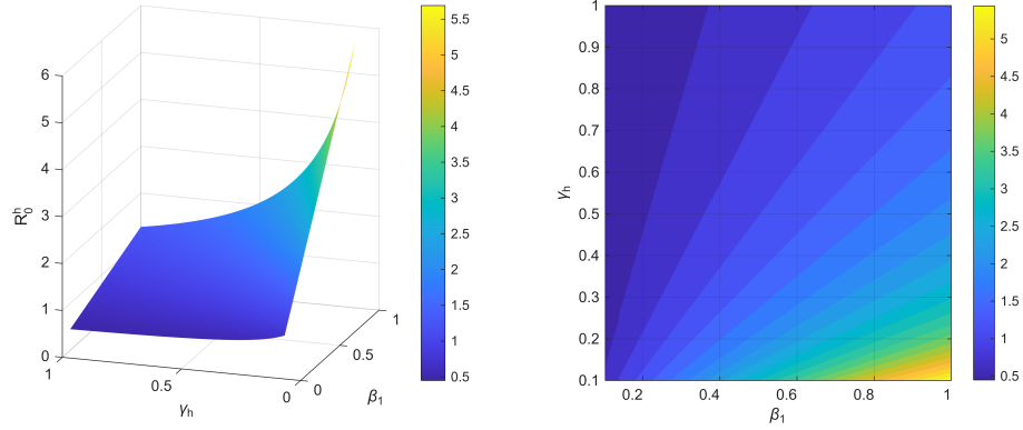
Figure 3: Influence of parameters \beta_1 and \gamma_h with respect to \mathcal{R}_0^h
