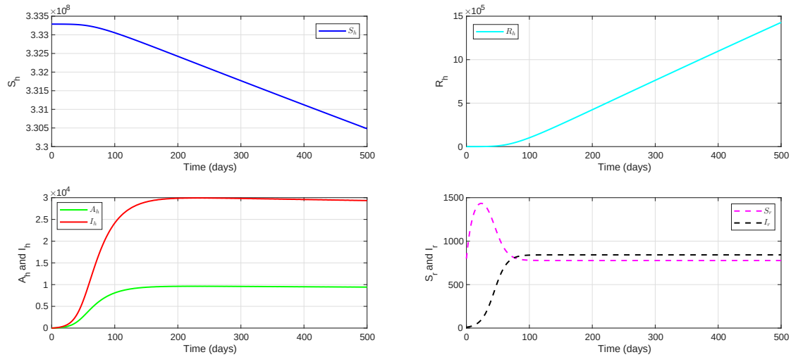
Figure 6: Dynamics of human and rodent populations
