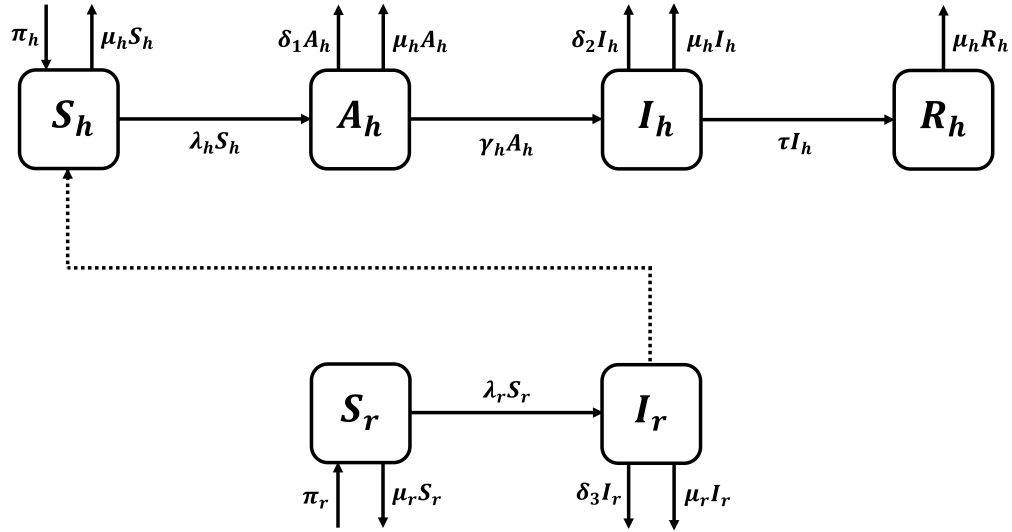
Figure 1: Mpox transmission diagram
