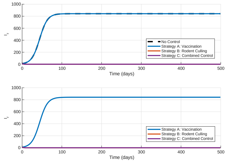
Figure 9: Dynamics of I_r under all control strategies
