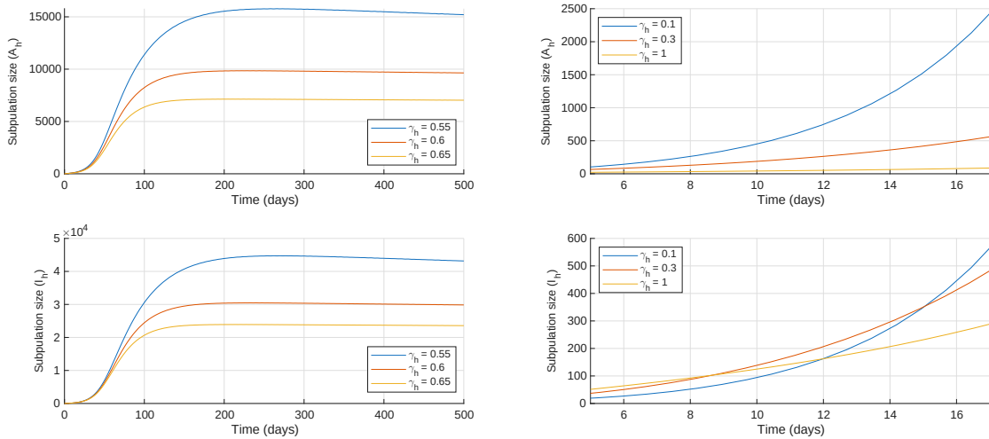
Figure 5: Influence of parameter \gamma_h with respect to A_h and I_h
