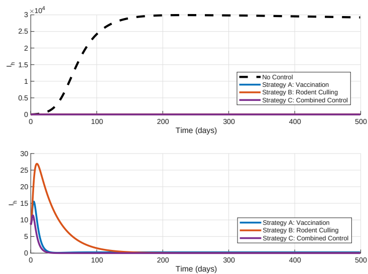
Figure 8: Dynamics of I_h under all control strategies
