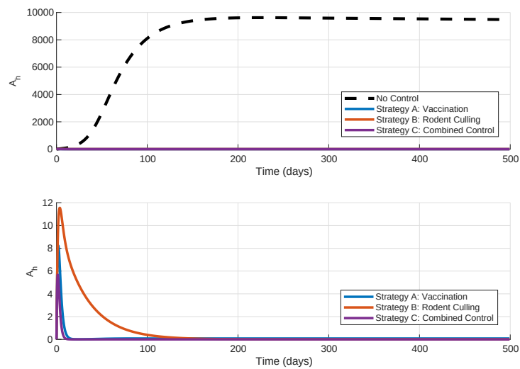
Figure 7: Dynamics of A_h under all control strategies
