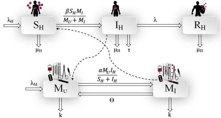
Figure 1: The compartmental model diagram.
